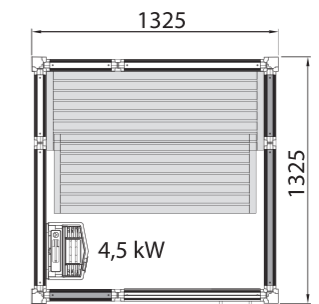
IMPRESSION-SAUNAKABINE IN 1313
