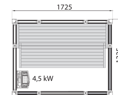
IMPRESSION-SAUNAKABINE IN 1713
